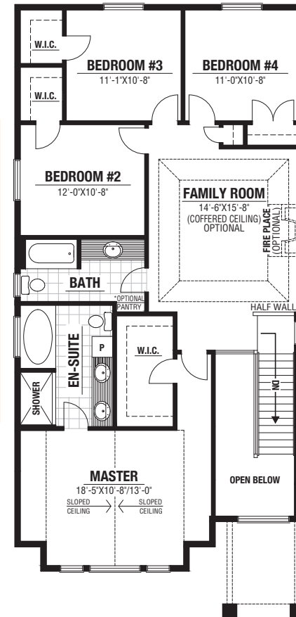
SECOND OPT. 3 1379 sq. ft.
